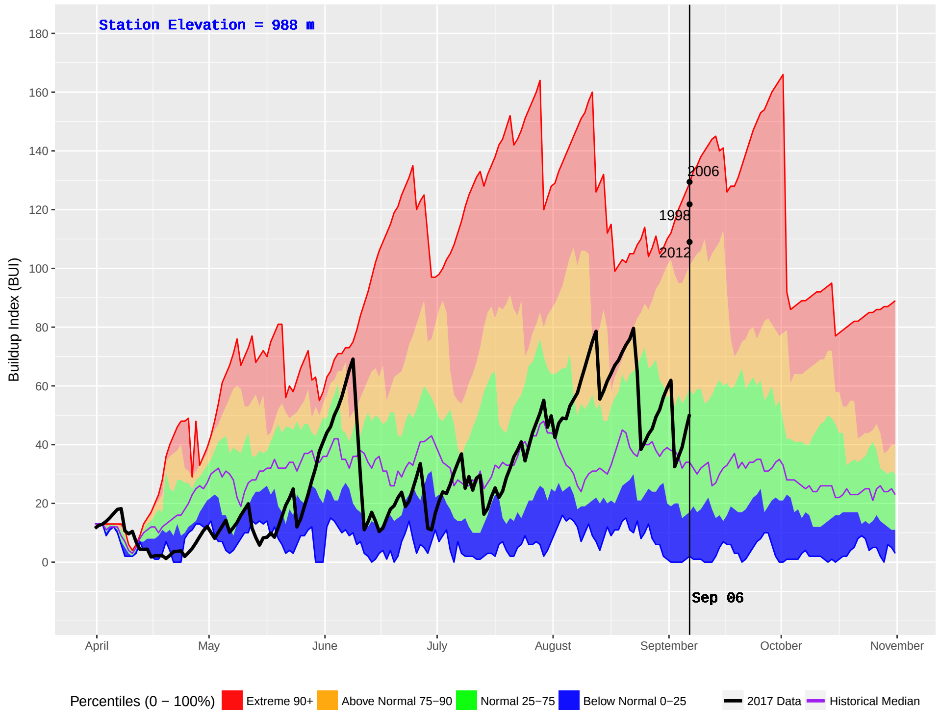
NOEL (437) : Historical (1993–2016) and Current (2017) Noon Buildup Index (BUI)
