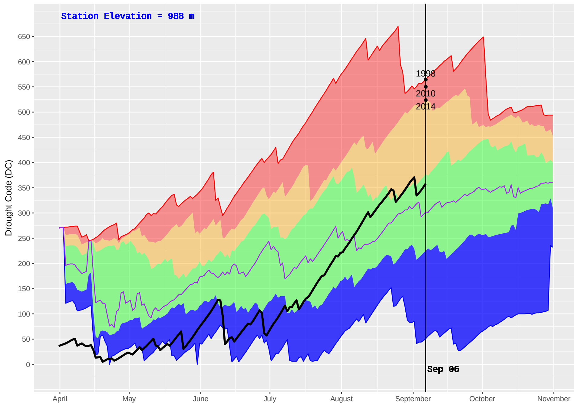
NOEL (437) : Historical (1993–2016) and Current (2017) Noon Drought Code (DC)
