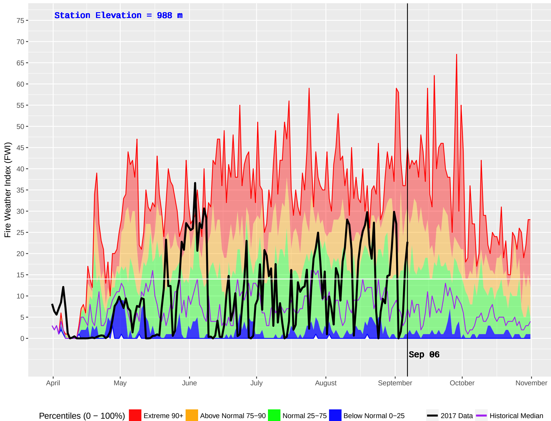
NOEL (437) : Historical (1993–2016) and Current (2017) Noon Fire Weather Index (FWI)
